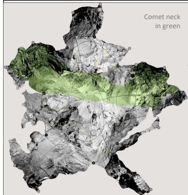
Figure 2: CSNB global map of 67P composed to show dust transport inward on the map.
